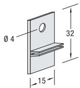
VA 8090 Hanger for top bar plastics
