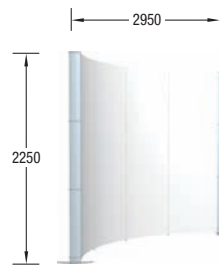
VA 5843 P1 4 panels with end caps in anodized aluminium
